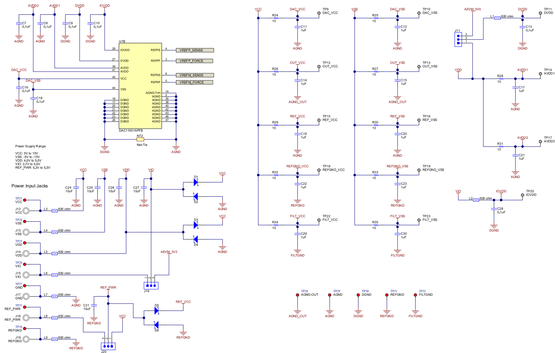
Figure 19. Schematic Page 4
