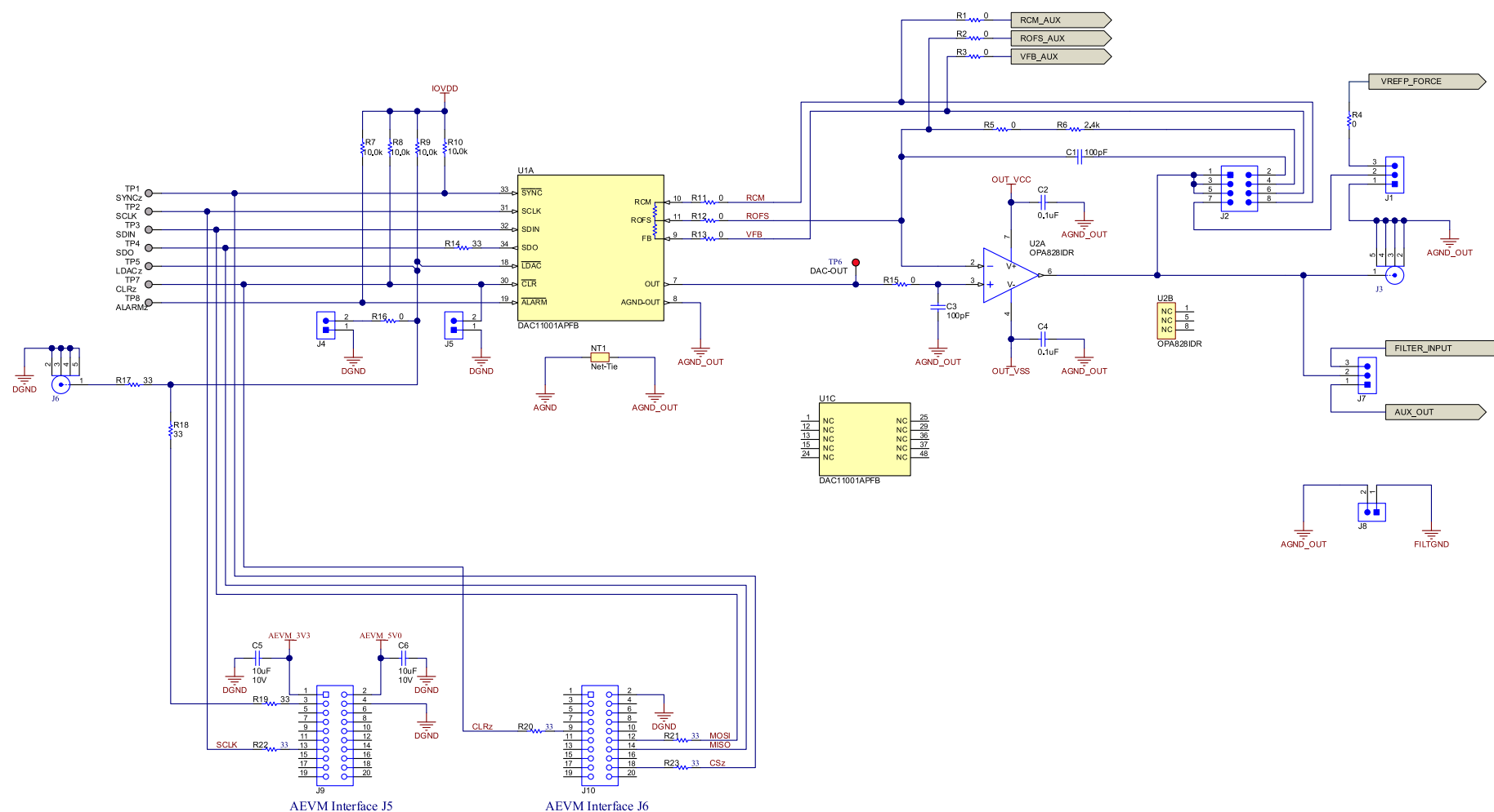
Figure 16. Schematic Page 1
