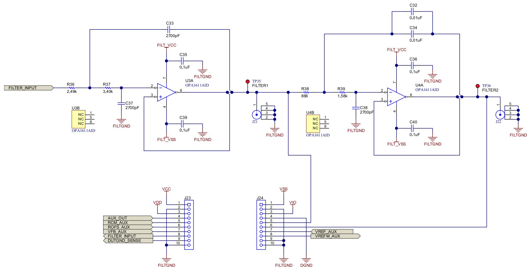
Figure 18. Schematic Page 3
