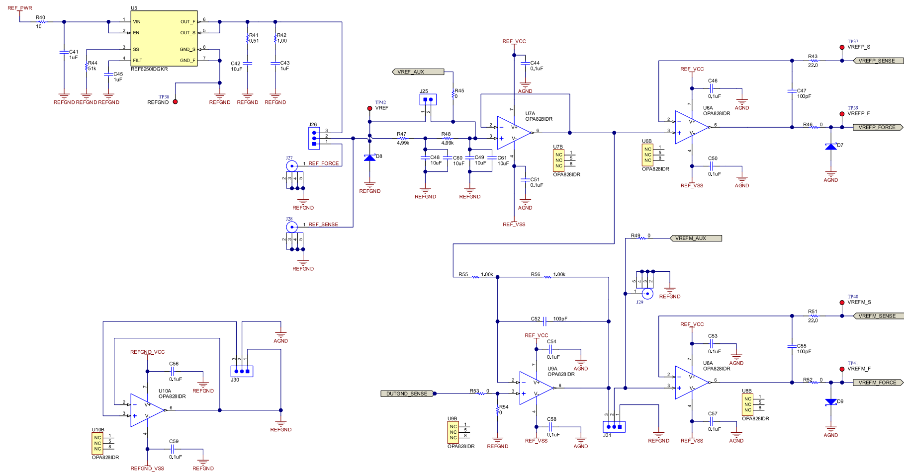
Figure 17. Schematic Page 2
