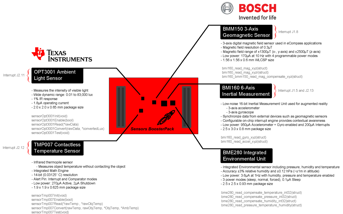
Figure 2. BOOSTXL-SENSORS Overview
