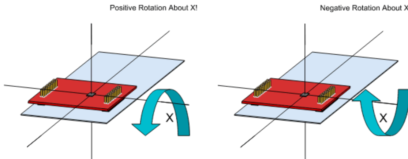
Figure 13. Rotation Around the X Axis
