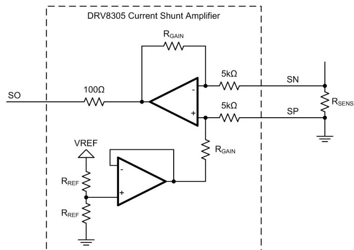
Figure 10. Current Sense
