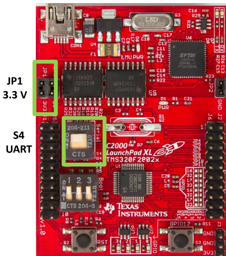
Figure 5. LAUNCHXL-F28027F Configurations
