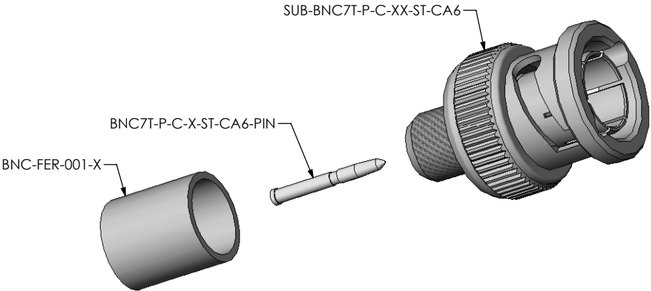
FIG.1 BNC7T-P-C-XX-ST-CA6 SHOWN
