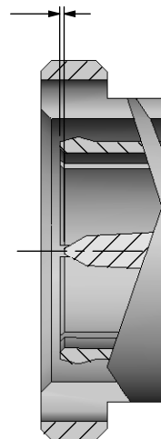
DETAIL 'A' SCALE 4:1
