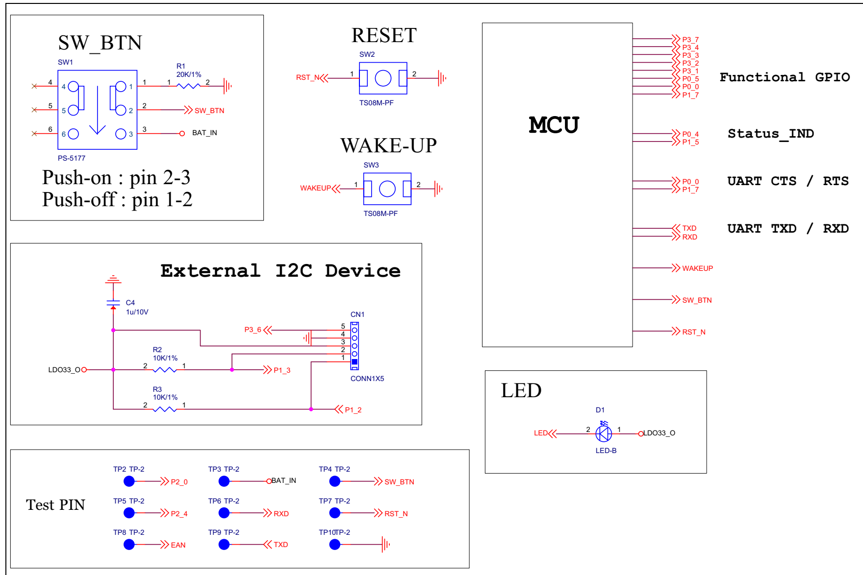
FIGURE 10-10: BM78SPP05MC2/NC2 REFERENCE CIRCUIT
