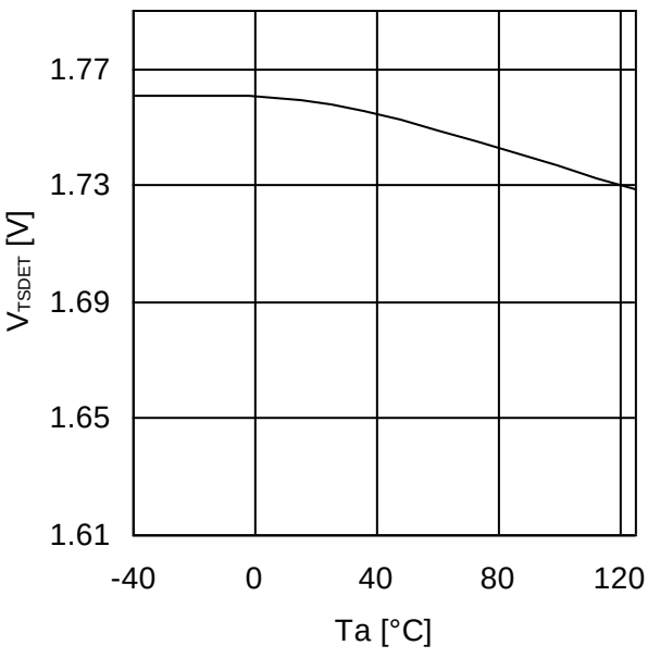
Figure 30. Thermal Detection Voltage
