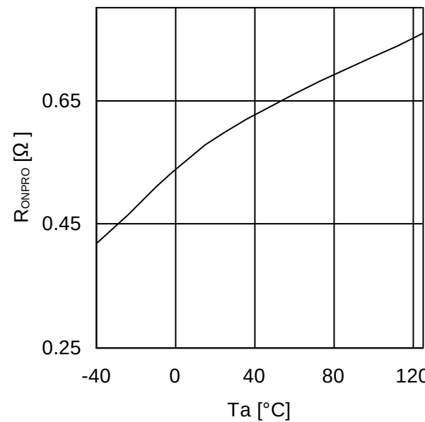
Figure 22. OUT2 ON-Resistance (I OUT2 =40mA)
