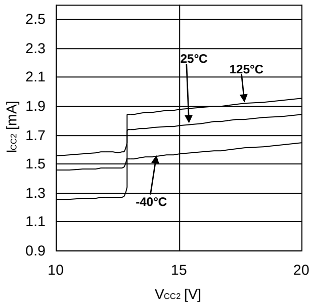
Figure 4. Output Side Circuit Current (MODE=H, VEE2=0V, OUT1=L)
