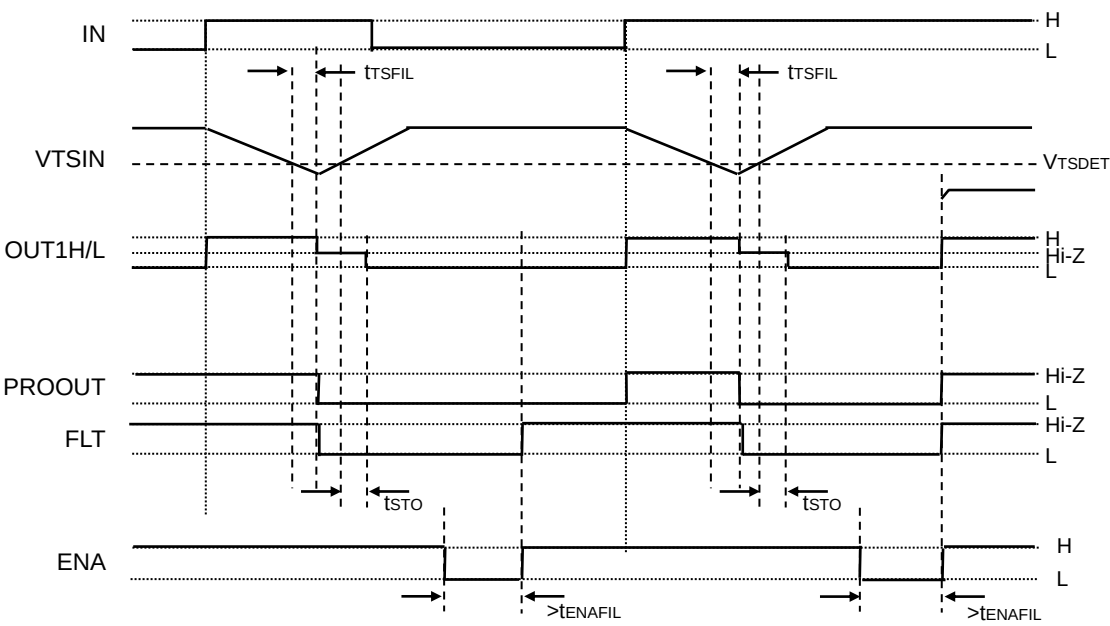
Figure 40. Thermal Protection Function Operation Timing Chart
