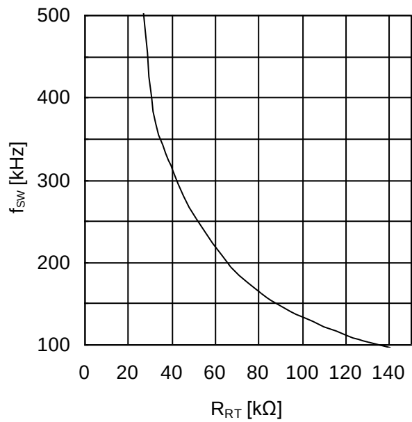
Figure 7. Oscillation Frequency
