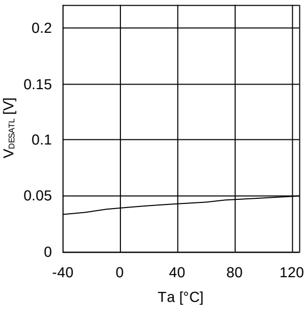
Figure 28. DESAT Low Voltage
