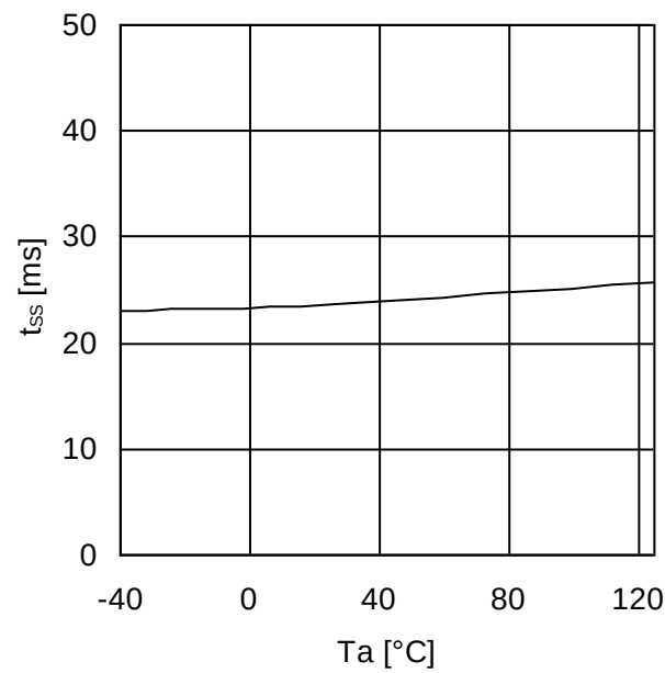
Figure 8. Soft-start Time
