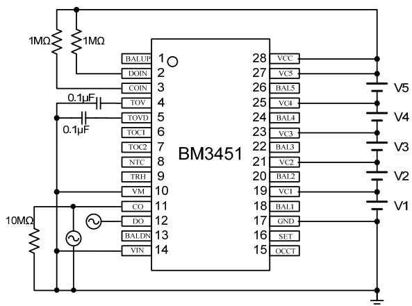
Test Circuit 2
