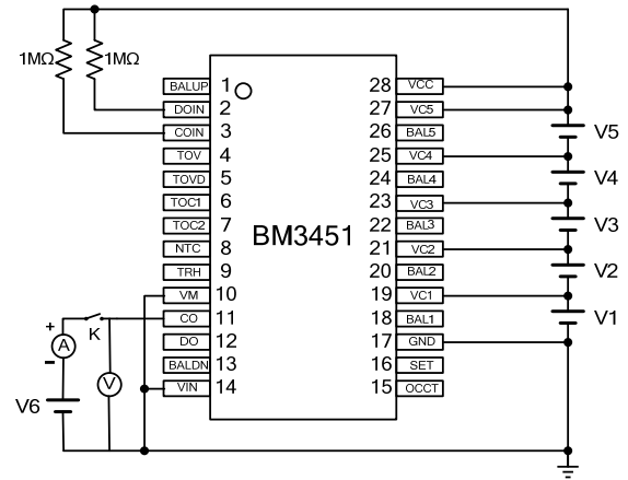
Test Circuit 6
