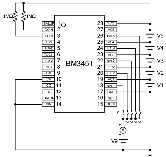
Test Circuit 8
