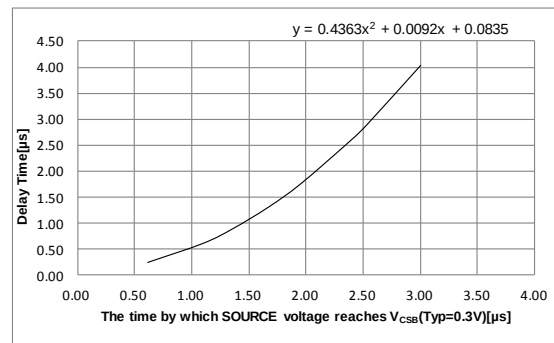
Figure 6B. Delay Time vs the Time by Which the SOURCE Pin Voltage Reaches V_{CSB} (Typ=0.3 V) (BM2P101FK-LB)
