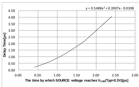
Figure 6C. Delay Time vs the Time by Which the SOURCE pin Voltage Reaches V_{CSB} (Typ=0.3 V) (BM2P131FK-LB)
