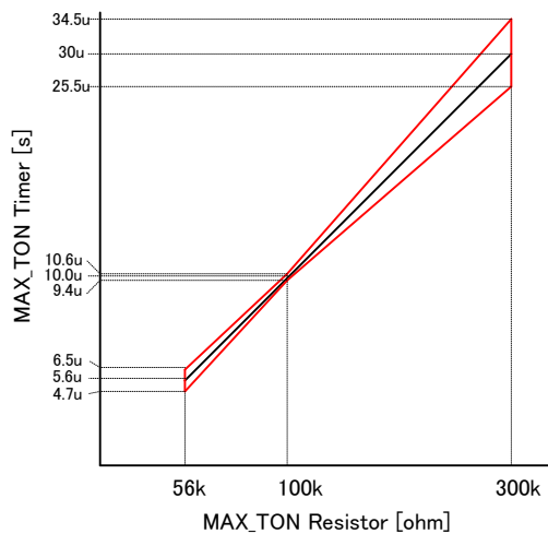
Figure 17. MAX_TON Timer vs MAX_TON Resistor( R_{\text{MAX\_TON}} )
