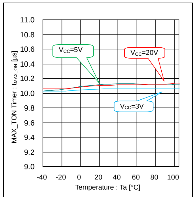
Figure 8. MAX_TON Timer vs Temperature ( R_{MAX\_TON}=100k\Omega , V_{DRAIN}=-0.3V \rightarrow V_{CC} \times 2 )
