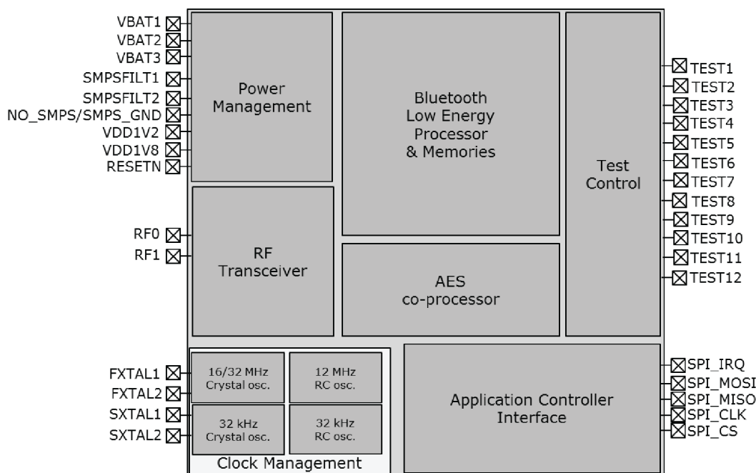
Figure 9. Block diagram
