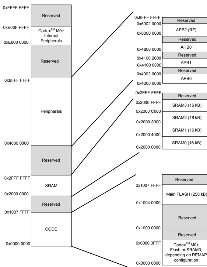
Figure 10. Memory map
