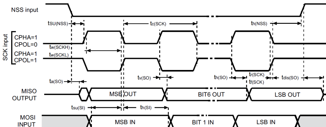
Figure 18. SPI timing diagram - slave mode and CPHA = 1
