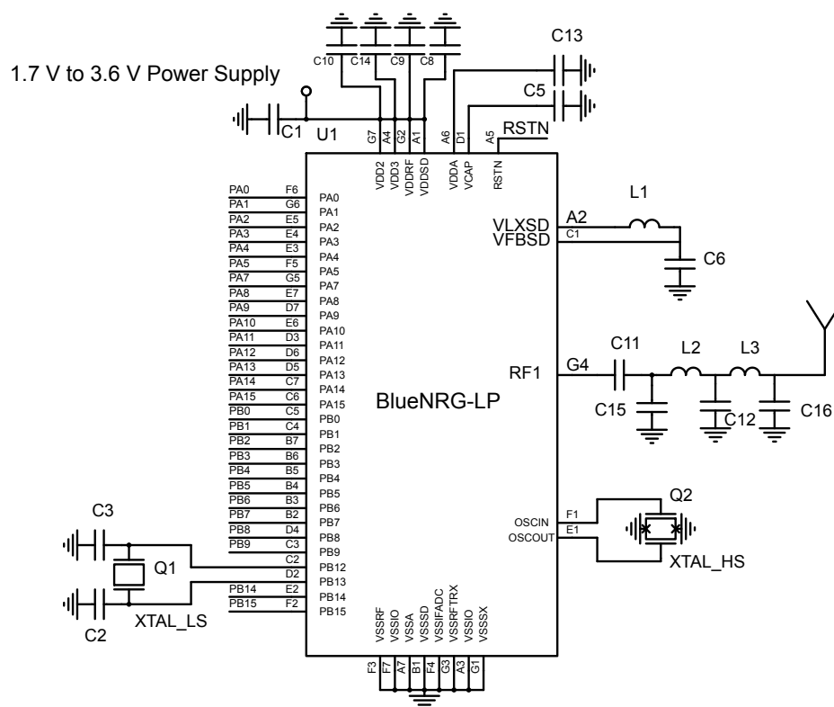
Figure 12. Application circuit: DC-DC converter, WCSP49 package
