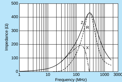
BLM21BD221SN1
