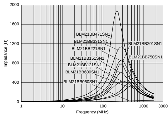
BLM21BB Series
