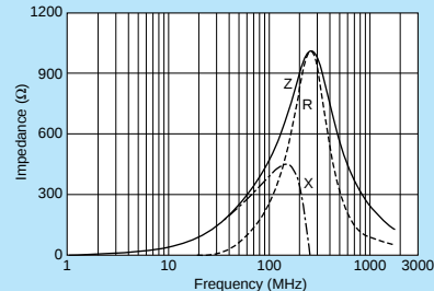
BLM21BD471SN1
