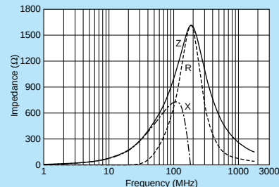
BLM21BD102SN1
