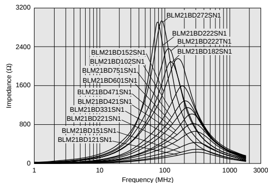
BLM21BD Series
