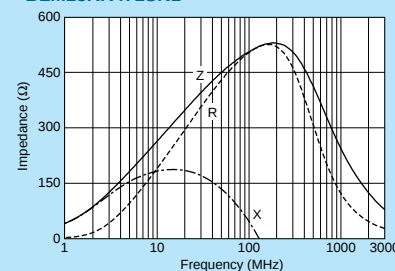
BLM18RK471SN1
