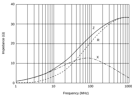
BLM21PG220SH1
