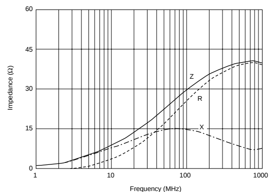
BLM21PG300SH1
