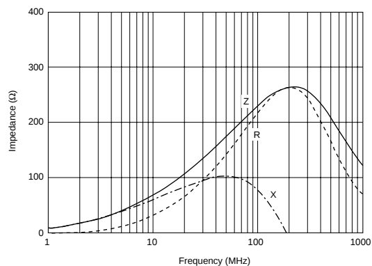
BLM21PG221SH1
