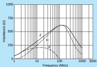
BLM21RK601SN1
