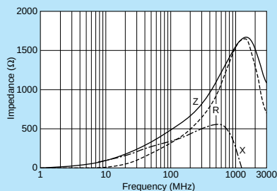
BLM18GG471SN1
