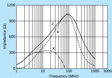
BLM21RK102SN1
