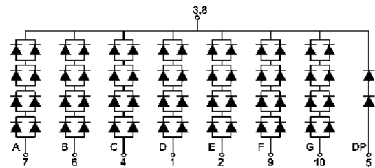
BL-S400F-11
