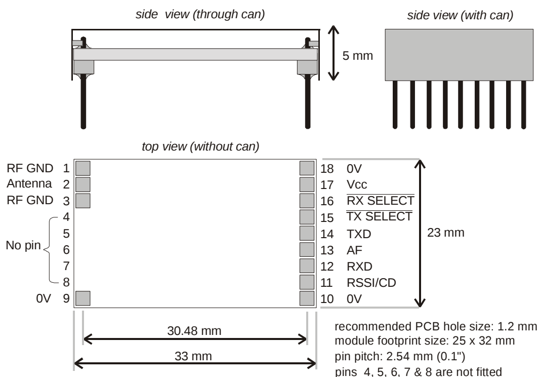
Fig. 2: Physical dimensions
