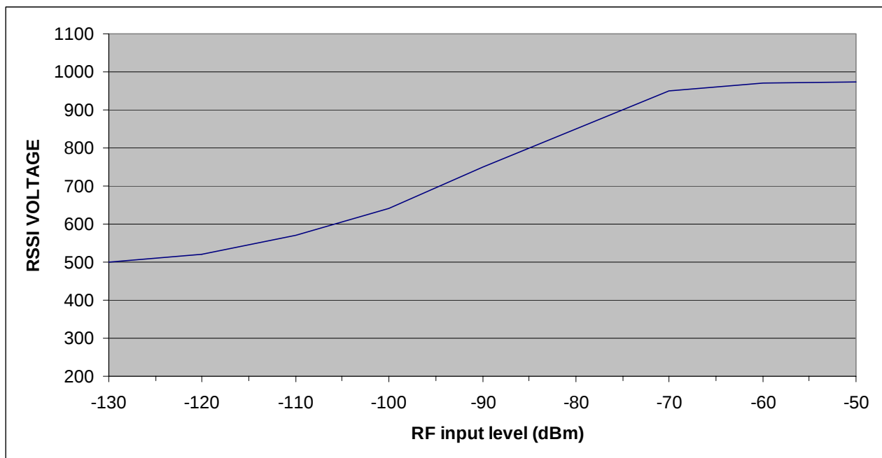
Figure 3: Typical RSSI
