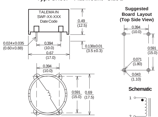
Type SH50F - Flat Mount - Size 2
