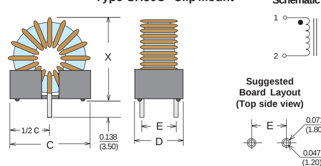
Type SH50C - Clip Mount
