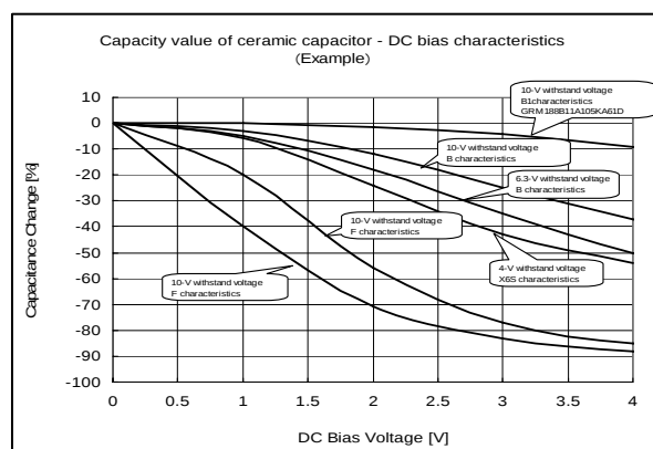
Figure 11. Capacity-bias characteristics
