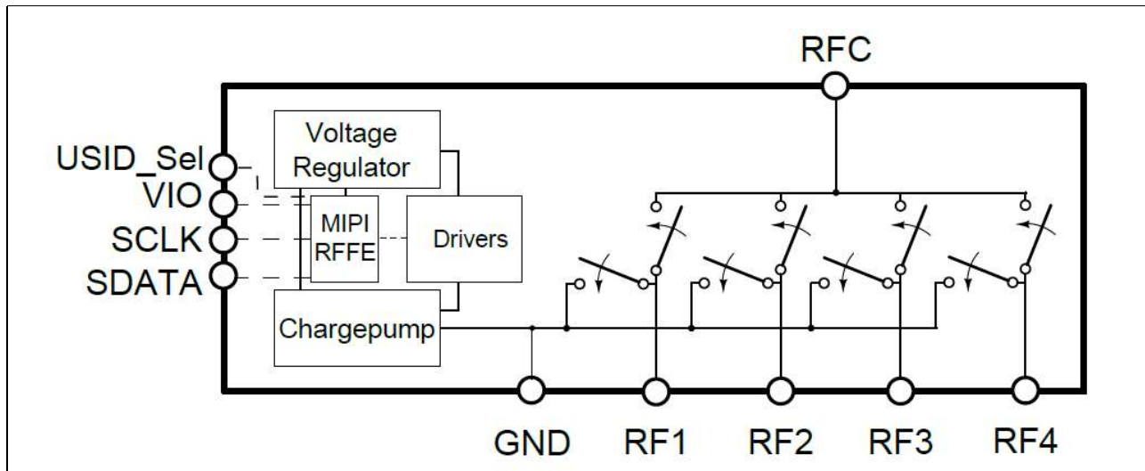
Figure 1 BGS143ML10 Block diagram
