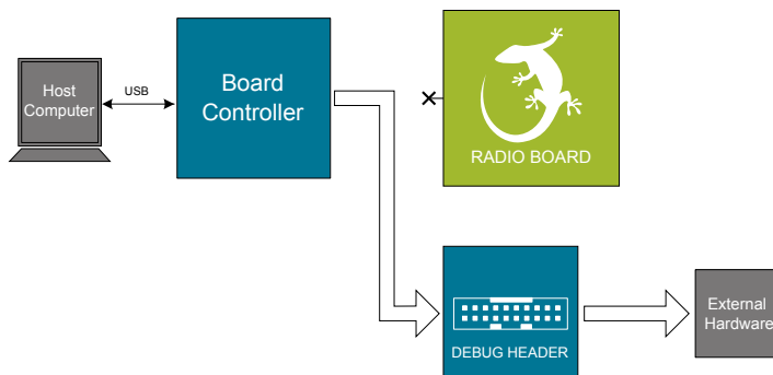
Figure 10.2. Debug OUT
