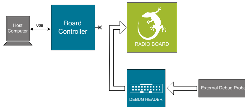
Figure 10.3. Debug IN
