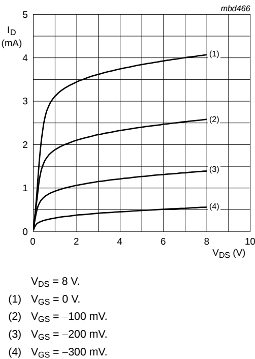
Fig 7. Typical output characteristics: BF861A.
