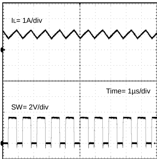
Figure 34. Switching Waveform ( V_{IN} = 3.3\text{V} , V_{OUT} = 1.8\text{V} , I_{OUT} = 1\text{A} , L = 1.5\mu\text{H} )
