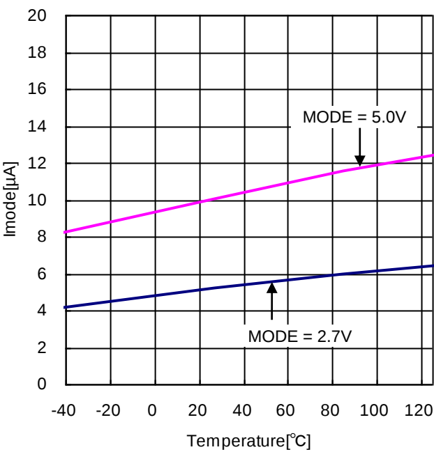
Figure 11. Mode Input Current vs Temperature
