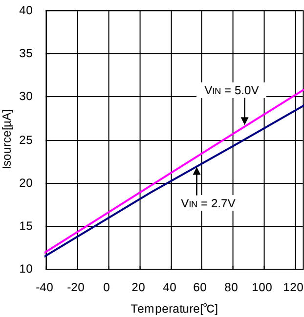
Figure 9. ITH Source Current vs Temperature
