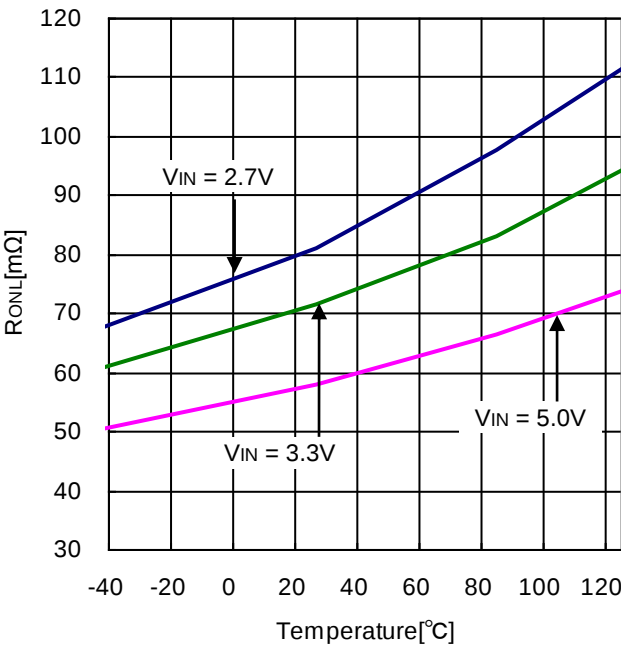
Figure 15. Low side FET ON-Resistance vs Temperature
