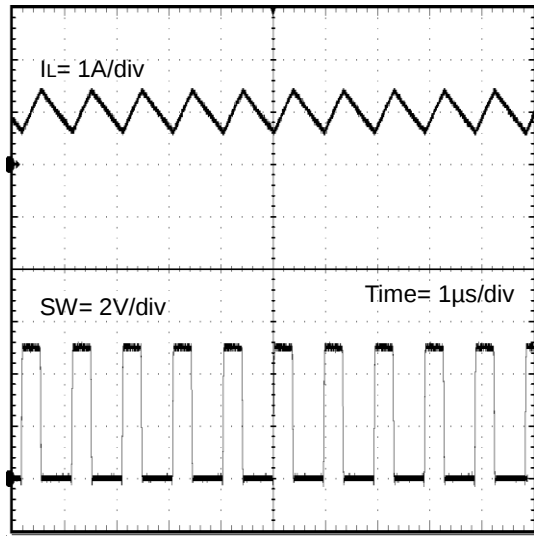
Figure 35. Switching Waveform ( V_{IN} = 5.0\text{V} , V_{OUT} = 1.8\text{V} , I_{OUT} = 1\text{A} , L = 1.5\mu\text{H} )
