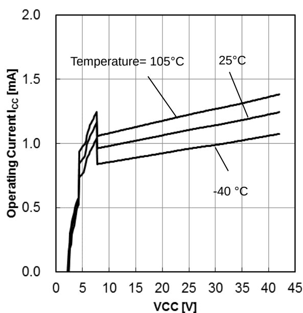
Figure 12. Operating Current vs Input Voltage ( V_{FB}= 1.2V )
