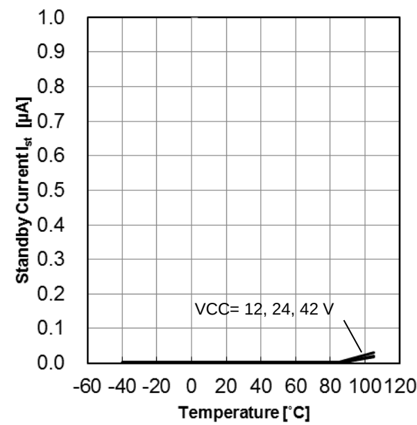
Figure 11. Standby Current vs Temperature
