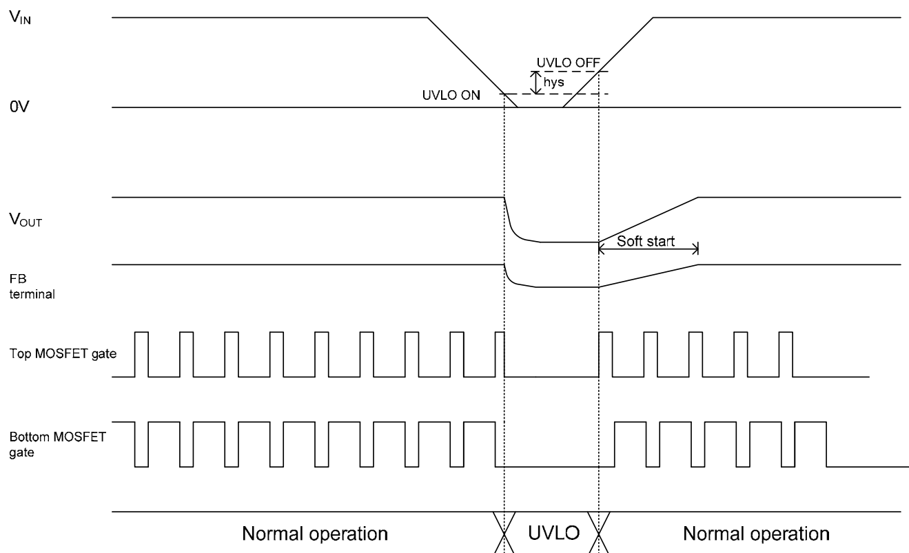
Figure 46. UVLO Timing Chart
