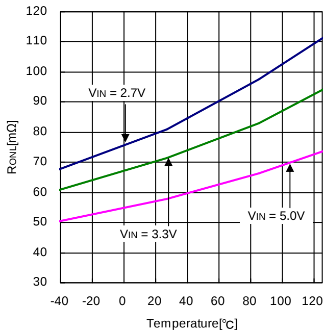
Figure 15. Low side FET ON-Resistance vs Temperature
