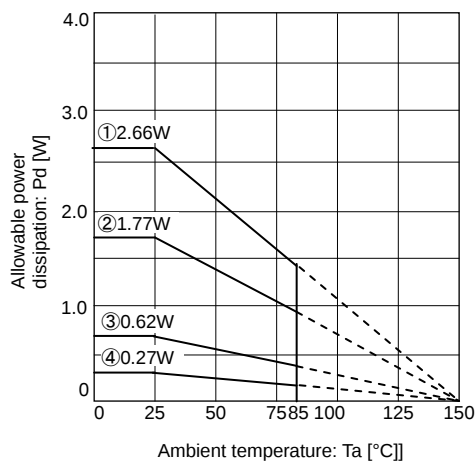
Figure 55. Thermal Derating Characteristics (VQFN016V3030)
