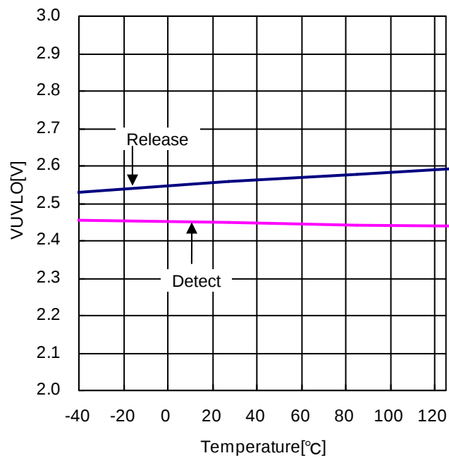
Figure 19. UVLO Threshold vs Temperature
