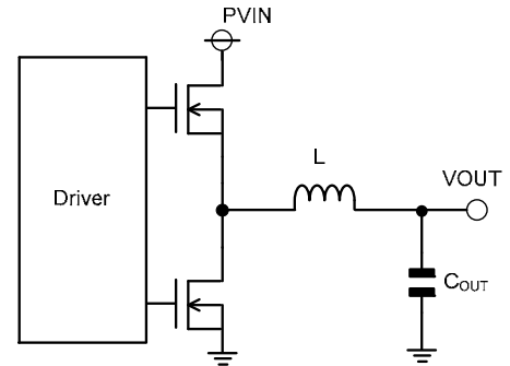
Figure 49. Output LC filter circuit
