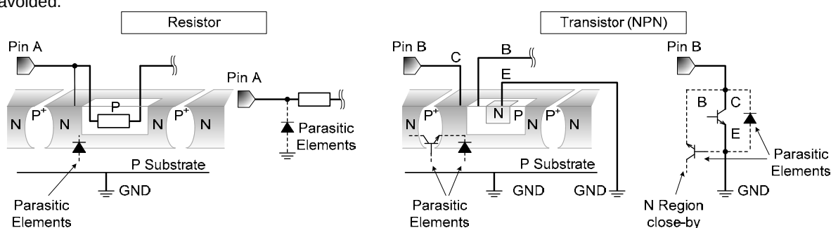
Figure 56. Example of monolithic IC structure
