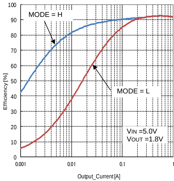
Figure 22. Efficiency vs Load Current ( V_{IN}=5V , V_{OUT}=1.8V , L=2.2\mu H )
