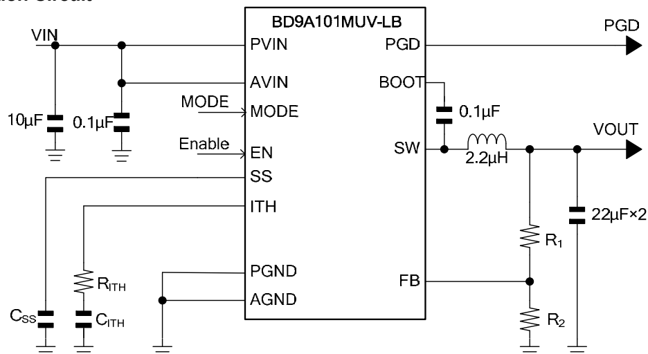
Figure 1. Application Circuit
