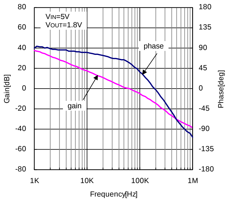
Figure 25. Closed Loop Response ( V_{IN}=5V , V_{OUT}=1.8V , I_{OUT}=1A , L=2.2\mu H , C_{OUT}=\text{Ceramic } 44\mu F )
