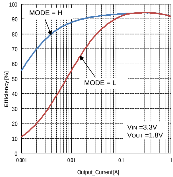
Figure 23. Efficiency vs Load Current ( V_{IN}=3.3V , V_{OUT}=1.8V , L=2.2\mu H )
