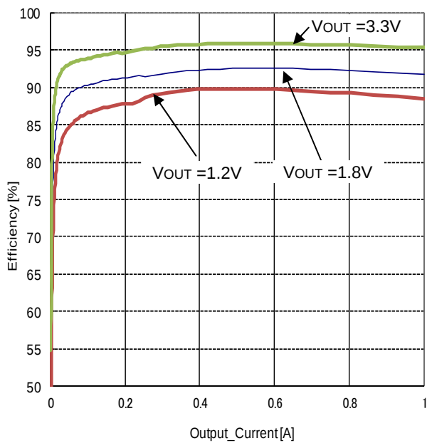
Figure 24. Efficiency vs Load Current ( V_{IN}=5.0V , MODE=5.0V , L=2.2\mu H )
