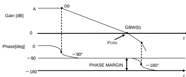
Figure 52. Bode Plot
