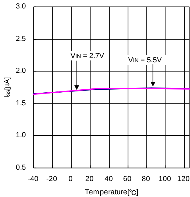
Figure 13. Soft Start Terminal Current vs Temperature
