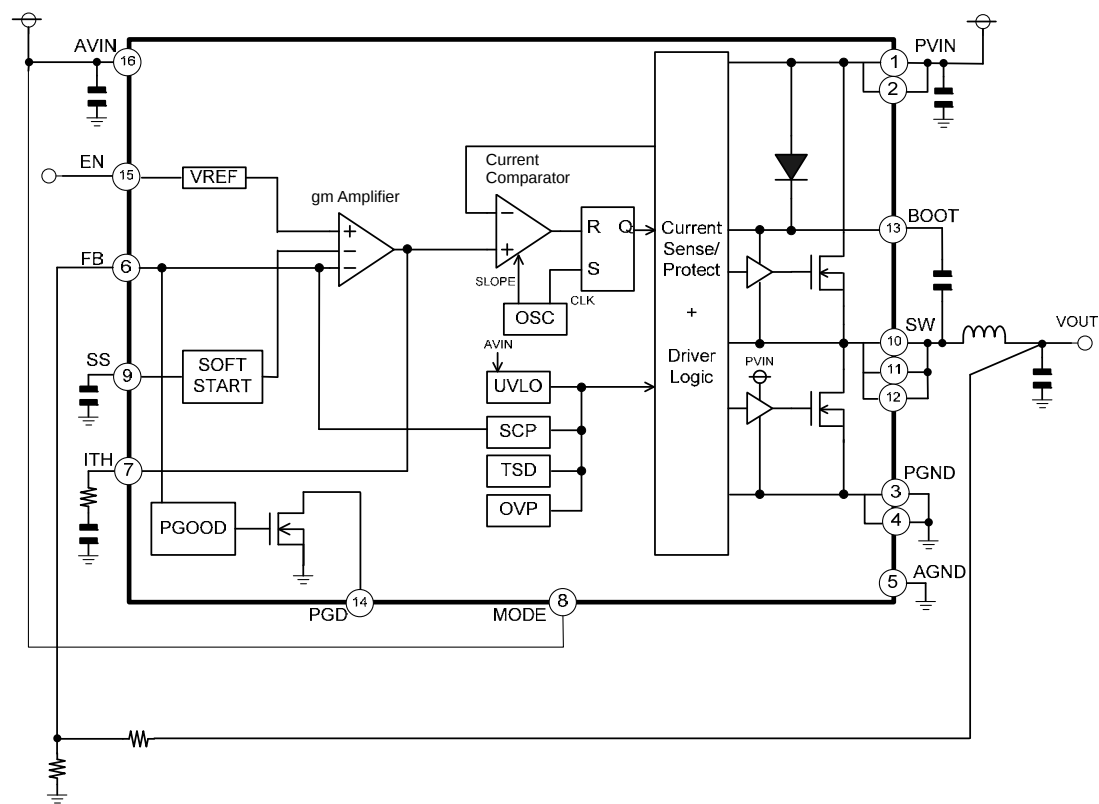
Figure 3. Block Diagram
