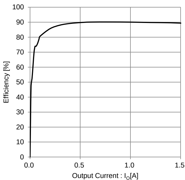
Figure 18. Efficiency vs Output Current (Conversion Efficiency 2 V_{IN} = 13.2 V)
