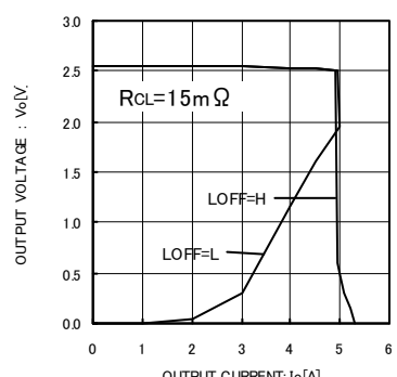
Fig.9 Load regulation
