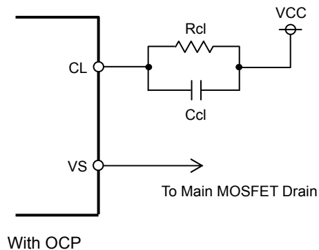
CL, VS Pin Connection
