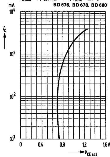
Collector-emitter saturation voltage V_{CEsat} = f(I_C) ; h_{FE} = 100 ; T_{case} = 25^\circ C
