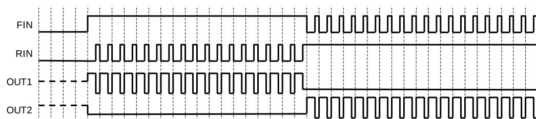
Figure 41. PWM Control Mode B Operation (Timing Chart)
