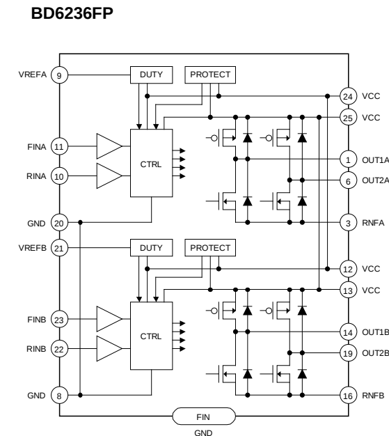
Figure 7. BD6236FP
