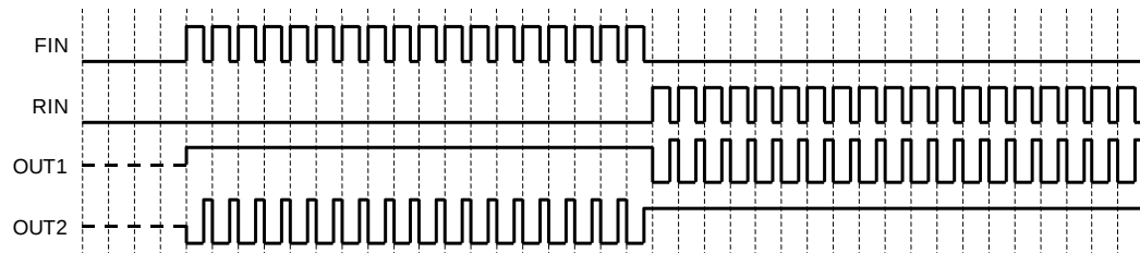
Figure 39. PWM Control Mode A Operation (Timing Chart)
