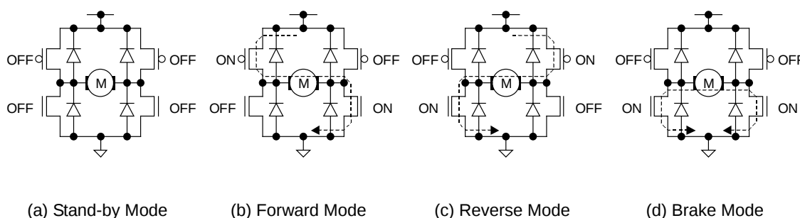
Figure 37. Four Basic Operations (Output Stage)
