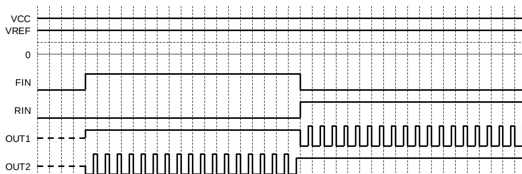
Figure 38. VREF Control Operation (Timing Chart)
