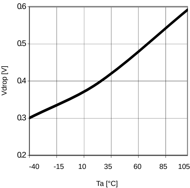
Figure 33. T_a - V_{drop} ( V_{CC}=6\text{V} , I_o=1\text{A} )
