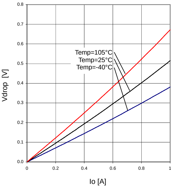
Figure 34. Minimum dropout Voltage 1 ( V_{CC}=4.5\text{V} )
