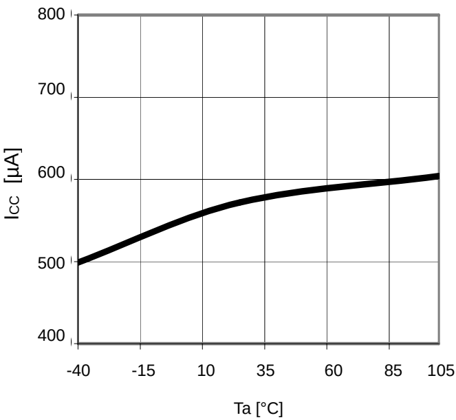
Figure 22. T_a - I_{CC}
