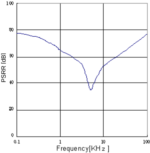
Figure 32. PSRR ( I_o=0\text{mA} )
