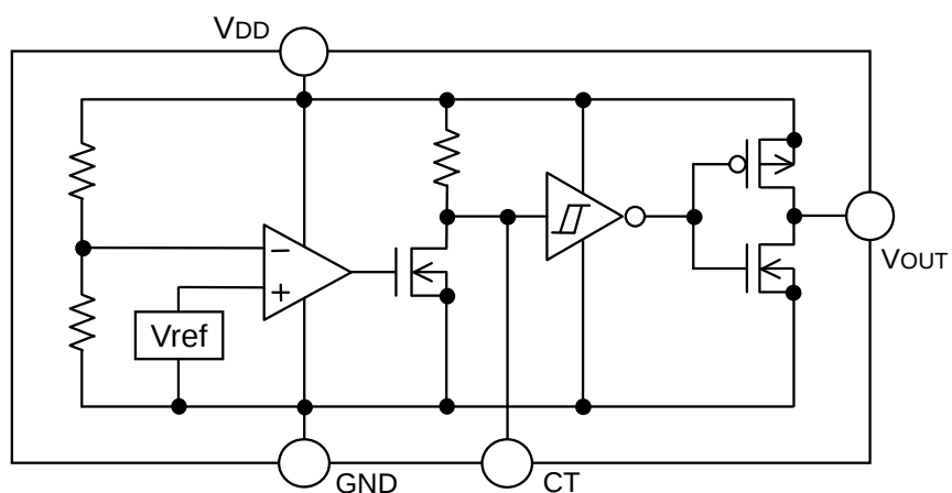
Figure.2 BD53Exxx-M Series
