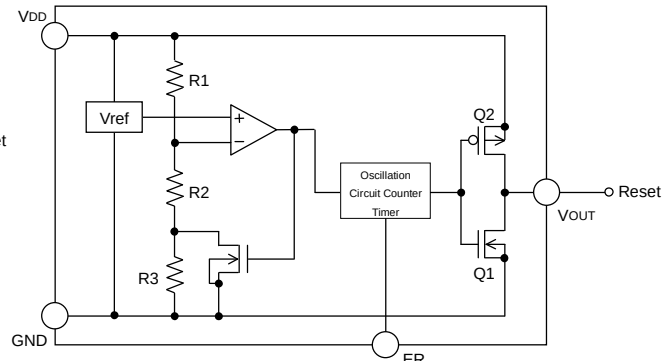
Fig.16 (BD46Exxxx-M Type Internal Block Diagram)
