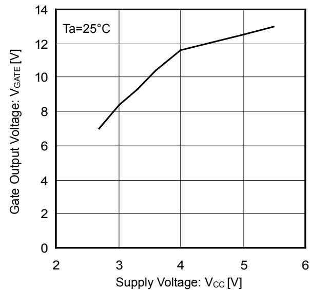
Figure 9. GATE Output Voltage vs Supply Voltage
