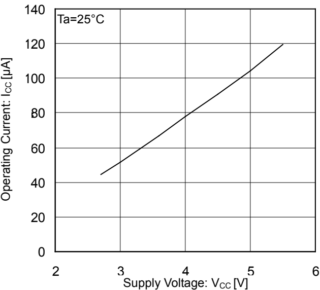
Figure 1. Operating Current vs Supply Voltage (AEN Enable)
