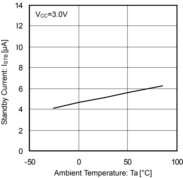
Figure 4. Standby Current vs Ambient Temperature (AEN Disable)
