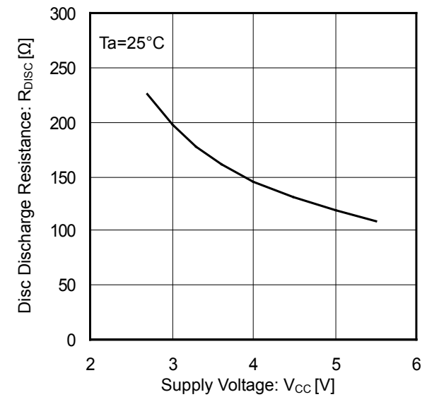
Figure 11. DISC Discharge Resistance vs Supply Voltage
