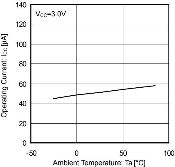
Figure 2. Operating Current vs Ambient Temperature (AEN Enable)
