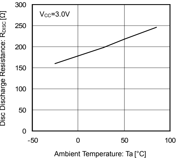
Figure 12. DISC Discharge Resistance vs Ambient Temperature
