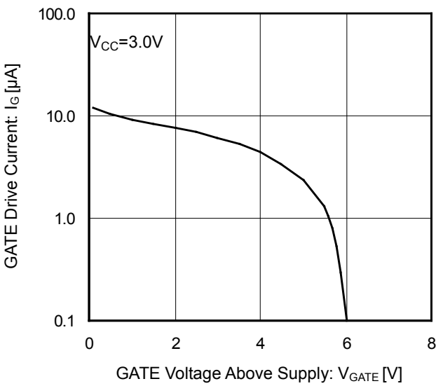
Figure 20. GATE Drive Current vs GATE Voltage Above Supply ( V_{CC} = 3V )
