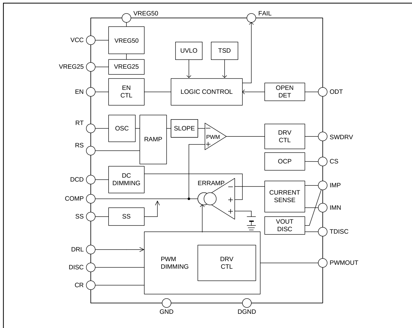
Figure 3. Block Diagram
