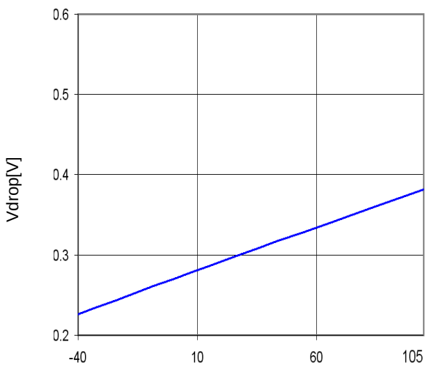
Figure 30. Minimum dropout Voltage1 (V cc =6V、I o =1.0A)
