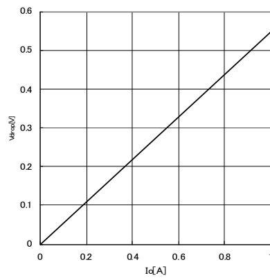
Fig.20 Minimum dropout Voltage 2 ( V_{cc}=4.5\text{V} , T_a=25^\circ\text{C} )
