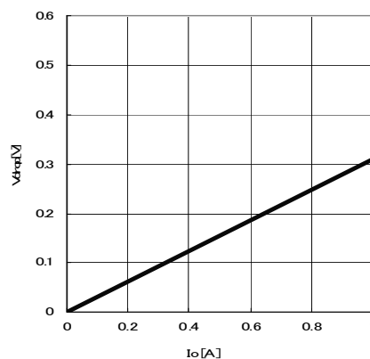
Fig.23 Minimum dropout Voltage 5 ( V_{cc}=10\text{V} , T_a=25^\circ\text{C} )
