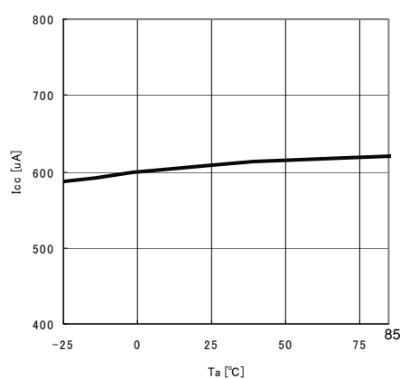
Fig.8 T_a - I_{cc}
