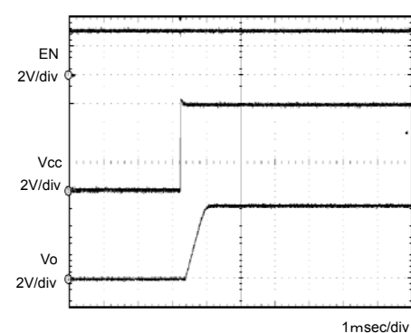
Fig.3 Input sequence 1 C_o=1\mu\text{F}
