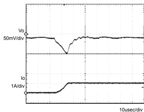
Fig.1 Transient Response (0→1.0A) C_o=1\mu\text{F}
