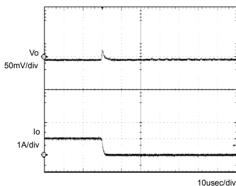
Fig.2 Transient Response (1.0→0A) C_o=1\mu\text{F}
