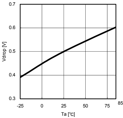
Fig.16 Minimum dropout Voltage 1 ( V_{cc}=5\text{V} , I_o=-1.0\text{A} )
