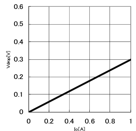
Fig.24 Minimum dropout Voltage 6 ( V_{cc}=12\text{V} , T_a=25^\circ\text{C} )
