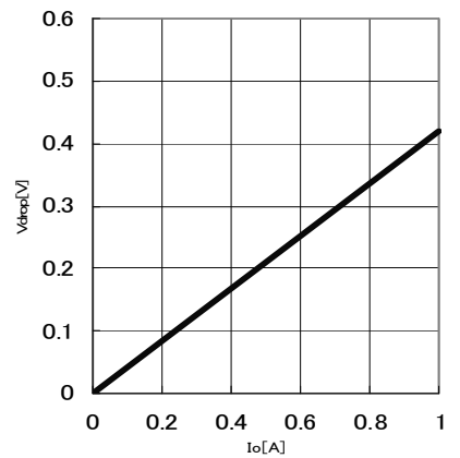
Fig.21 Minimum dropout Voltage 3 ( V_{cc}=6\text{V} , T_a=25^\circ\text{C} )
