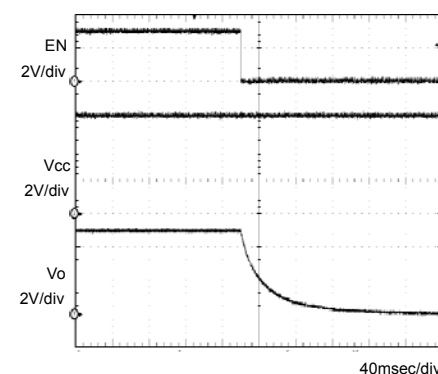
Fig.6 OFF sequence 2 C_o=1\mu\text{F}
