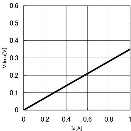
Fig.22 Minimum dropout Voltage 4 ( V_{cc}=8\text{V} , T_a=25^\circ\text{C} )
