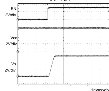
Fig.5 Input sequence 2 C_o=1\mu\text{F}
