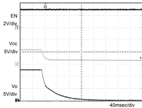
Fig.4 OFF sequence 1 C_o=1\mu\text{F}
