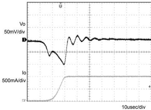
Fig.1 Transient Response (0→1A) C_o=1\mu\text{F}
