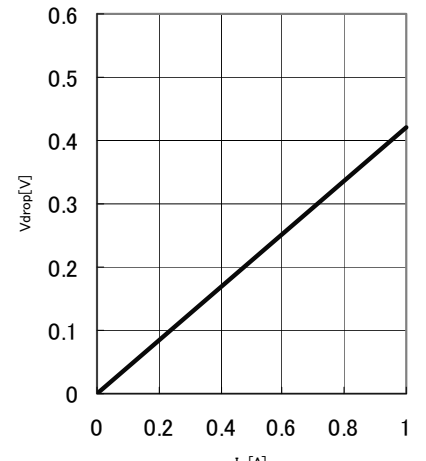
Fig.21 Minimum dropout Voltage 3 ( V_{cc}=6 V, T_a=25^\circ\text{C} )
