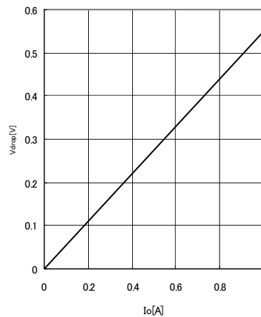
Fig.20 Minimum dropout Voltage 2 ( V_{cc}=4.5 V, T_a=25^\circ\text{C} )
