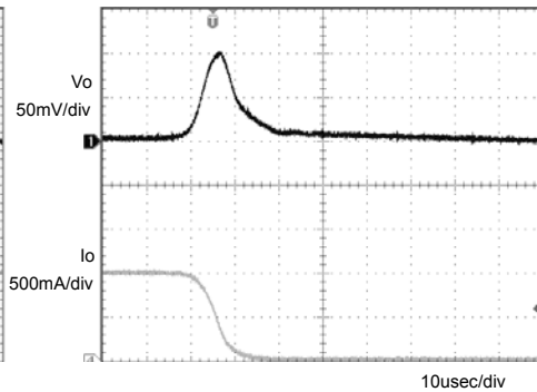
Fig.2 Transient Response (1→0A) C_o=1\mu\text{F}
