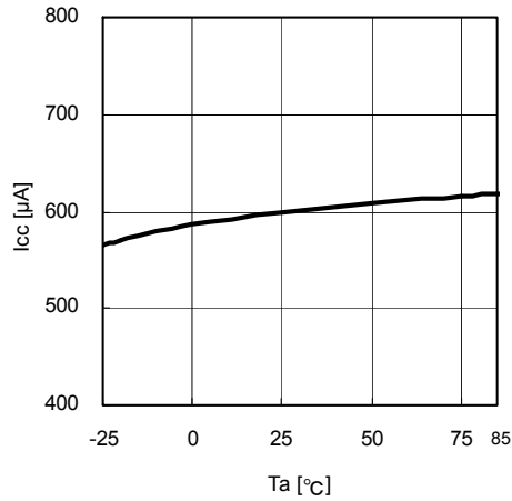
Fig.8 T_a - I_{CC}
