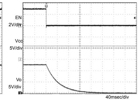
Fig.6 OFF sequence 2 C_o=1\mu\text{F}
