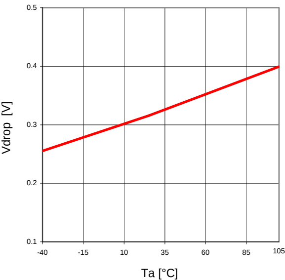
Figure 33. Ta-Vdrop (Vcc=6V, Io=0.3A)
