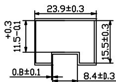
TUBE MECHANICAL DIMENSION
