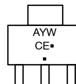
SOT-223 (TO-261) CASE 318E STYLE 1
