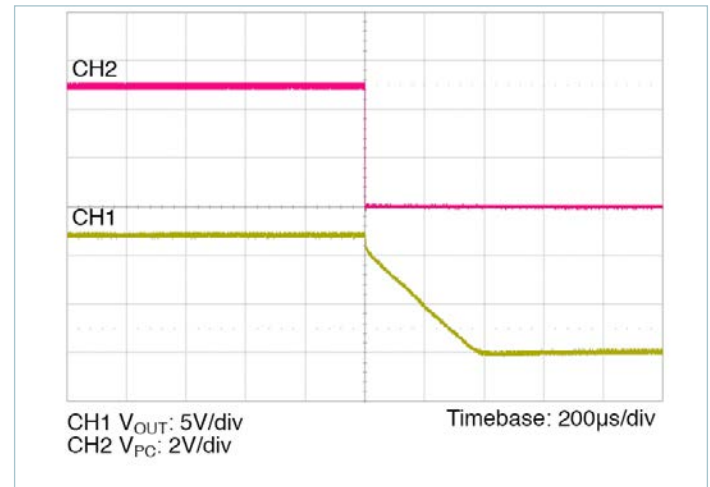
Figure 17 — PC disable wave form; V_{IN} = 352V , C_{OUT} = 1000\mu F , full load
