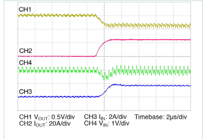
Figure 15 — 0A – 25A transient response: C_{IN} = 330\mu F , I_{IN} measured prior to C_{IN} , no external C_{OUT}
