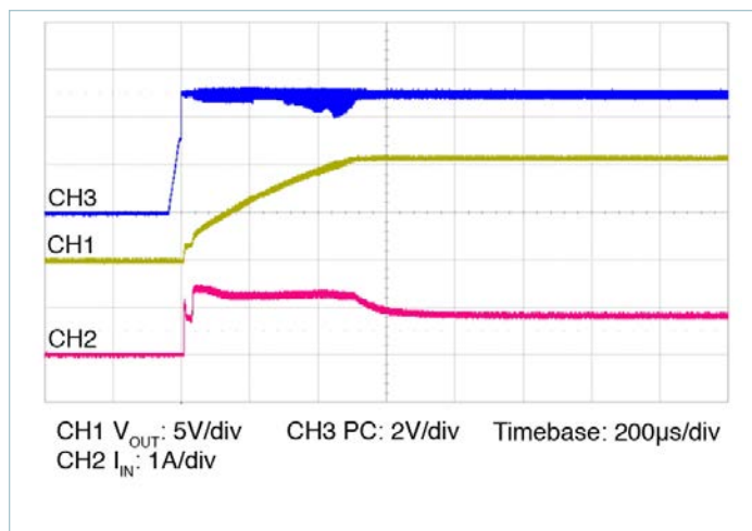
Figure 14 — Start up from application of PC; V_{IN} pre-applied C_{OUT} = 1200\mu F
