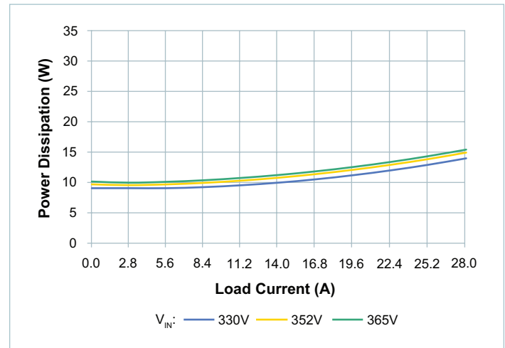
Figure 6 — Power dissipation at T_{CASE} = -40^{\circ}\text{C}
