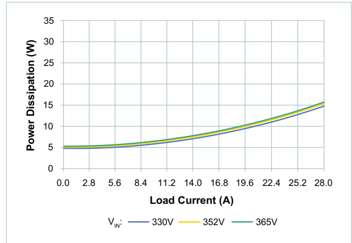
Figure 10 — Power dissipation at T_{CASE} = 100^{\circ}\text{C}
