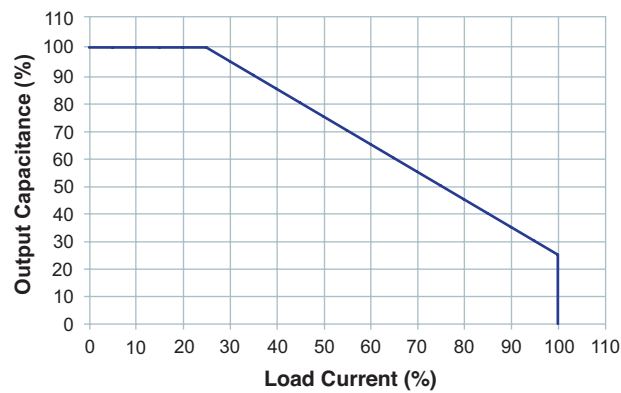
Figure 2 — Start up load current vs. output capacitance
