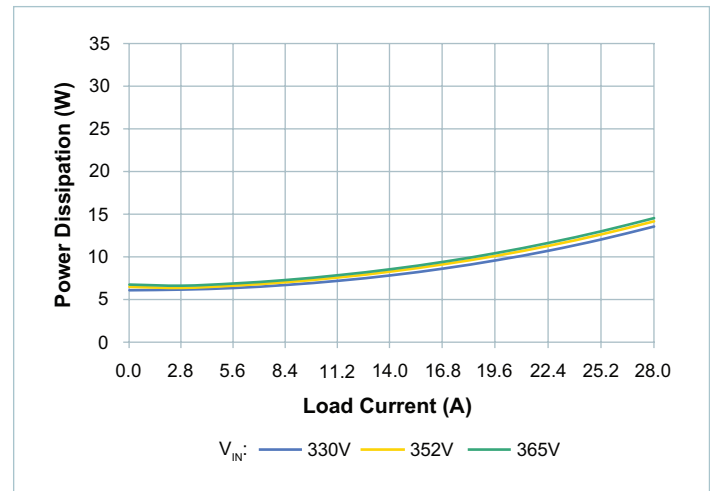
Figure 8 — Power dissipation at T_{CASE} = 25^{\circ}\text{C}
