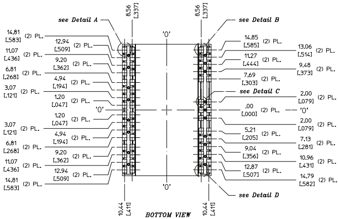
BOTTOM VIEW
