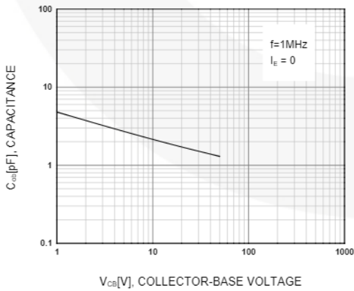
Figure 5. Output Capacitance
