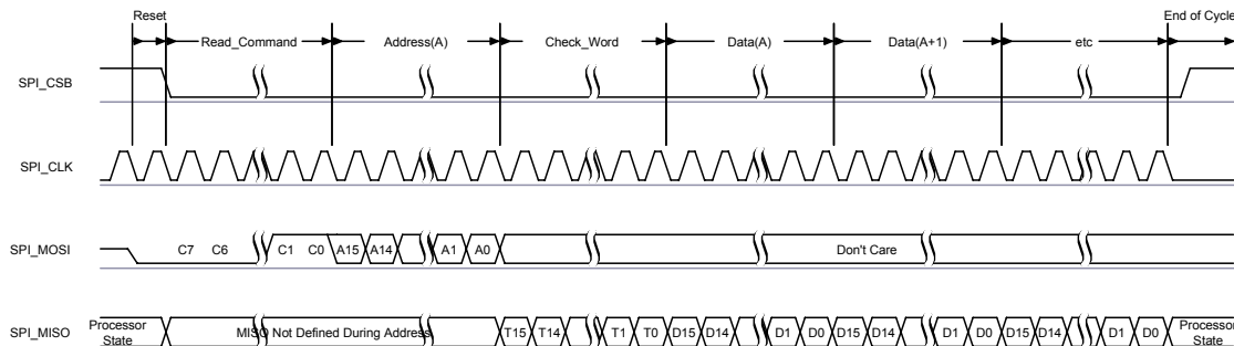
Figure 11.16: Read Operation
