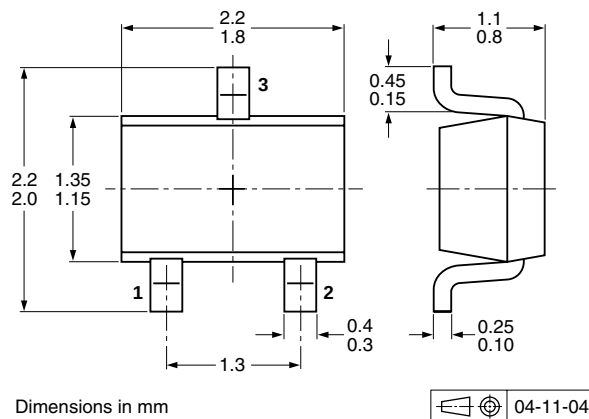
Fig 9. Package outline BAV99W (SOT323/SC-70)
