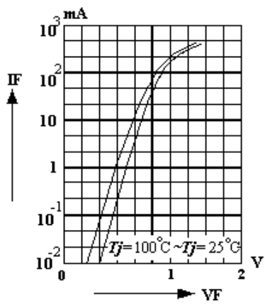
Forward characteristics
