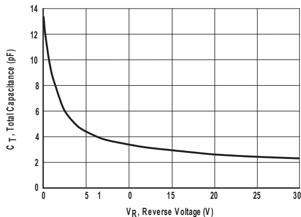
Figure 4. Total Capacitance
