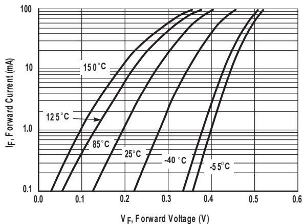
Figure 2. Forward Voltage
