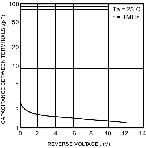
FIG.3-TYPICAL TERMINALS CAPACITANCE
