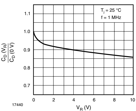
Figure 4. Relative Capacitance vs. Reverse Voltage
